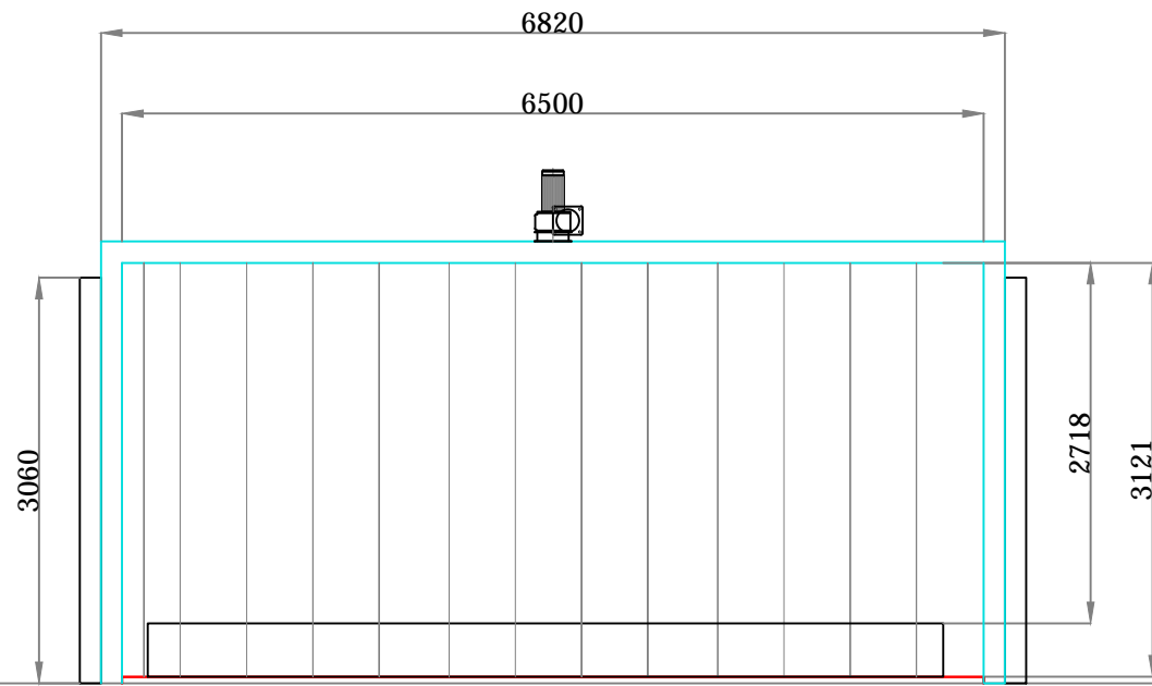
Curing Oven Side Sections
